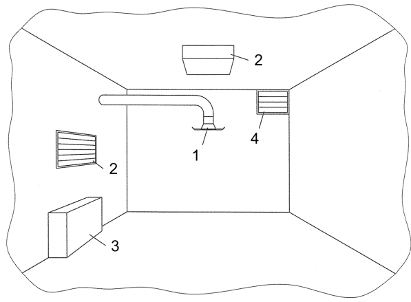
Figure 16. Solid angle \Omega depending on location of duct outlet
