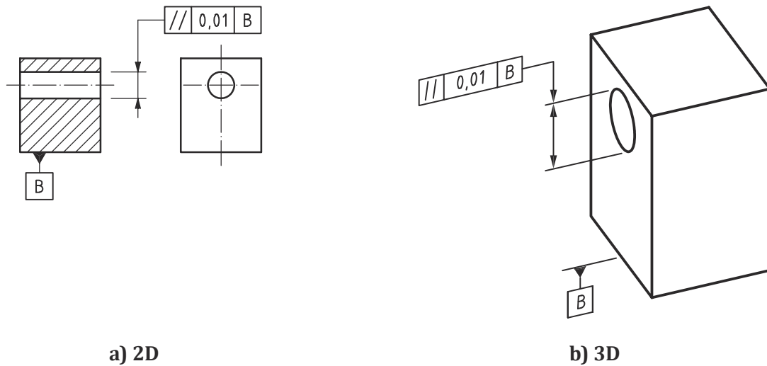
Figure 120 — Parallelism indication
